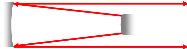
Unstable confocal resonator, g_1 g_2 > 1
